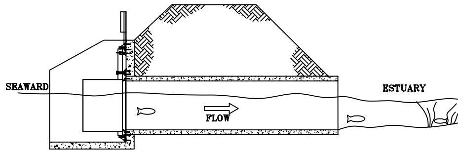
RISING TIDE ALLOWING INCOMING TIDE TO FLOOD ESTUARY BASIN
