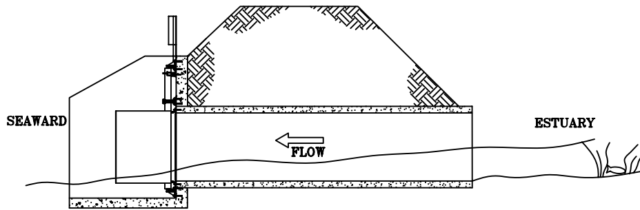
GH-850-R ACTING AS NORMAL FLAP GATE ALLOWING ESTUARY DRAINAGE
