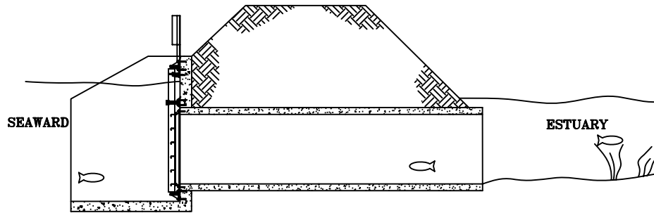
GH-850-R CLOSES AT SET LEVEL LIMITING ESTUARY FLOOD LEVEL
