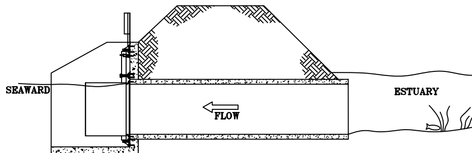
GH-850-R OPENS WHEN TIDE LEVEL IS LOWER THAN ESTUARY LEVEL
